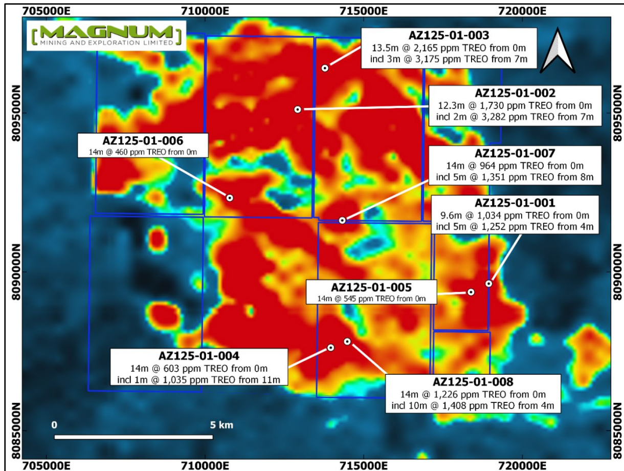
Figure 1 - Piracanjuba North Target auger hole locations and intercepts. Blue outline are Magnum's leases. Background is an image of the thorium channel of an airborne geophysical survey.
